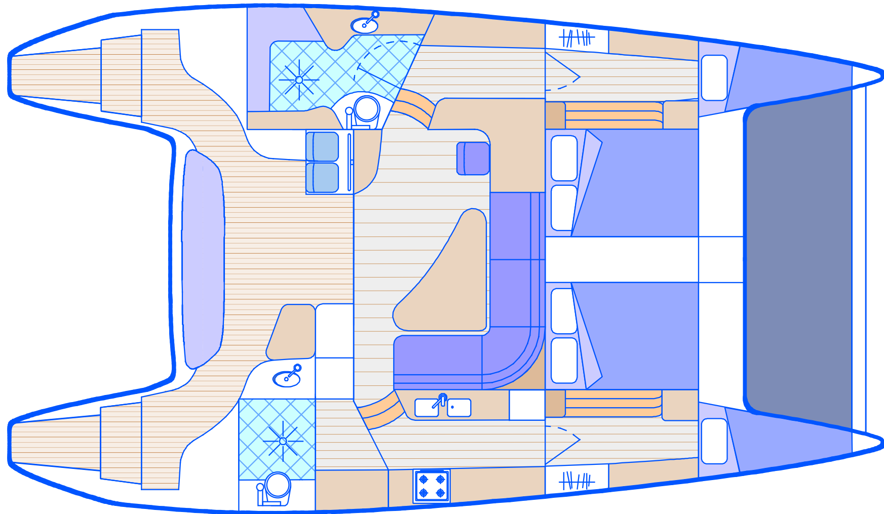
LIGHTWAVE 38 ACCOM OPTION -2 NAV STN LOOKING FWD WITH OTIONAL SECOND TOILET AND SHWR TO STBD
