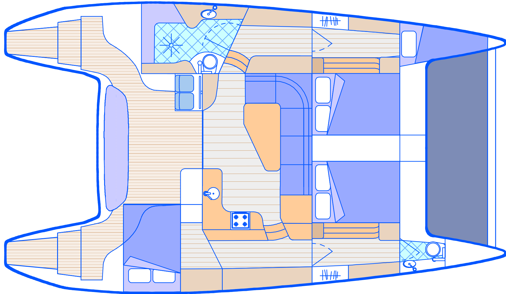
LIGHTWAVE 38 ACCOM OPTION -4 UPSTAIRS GALLEY WITH OPTIONAL FWD TOILET
