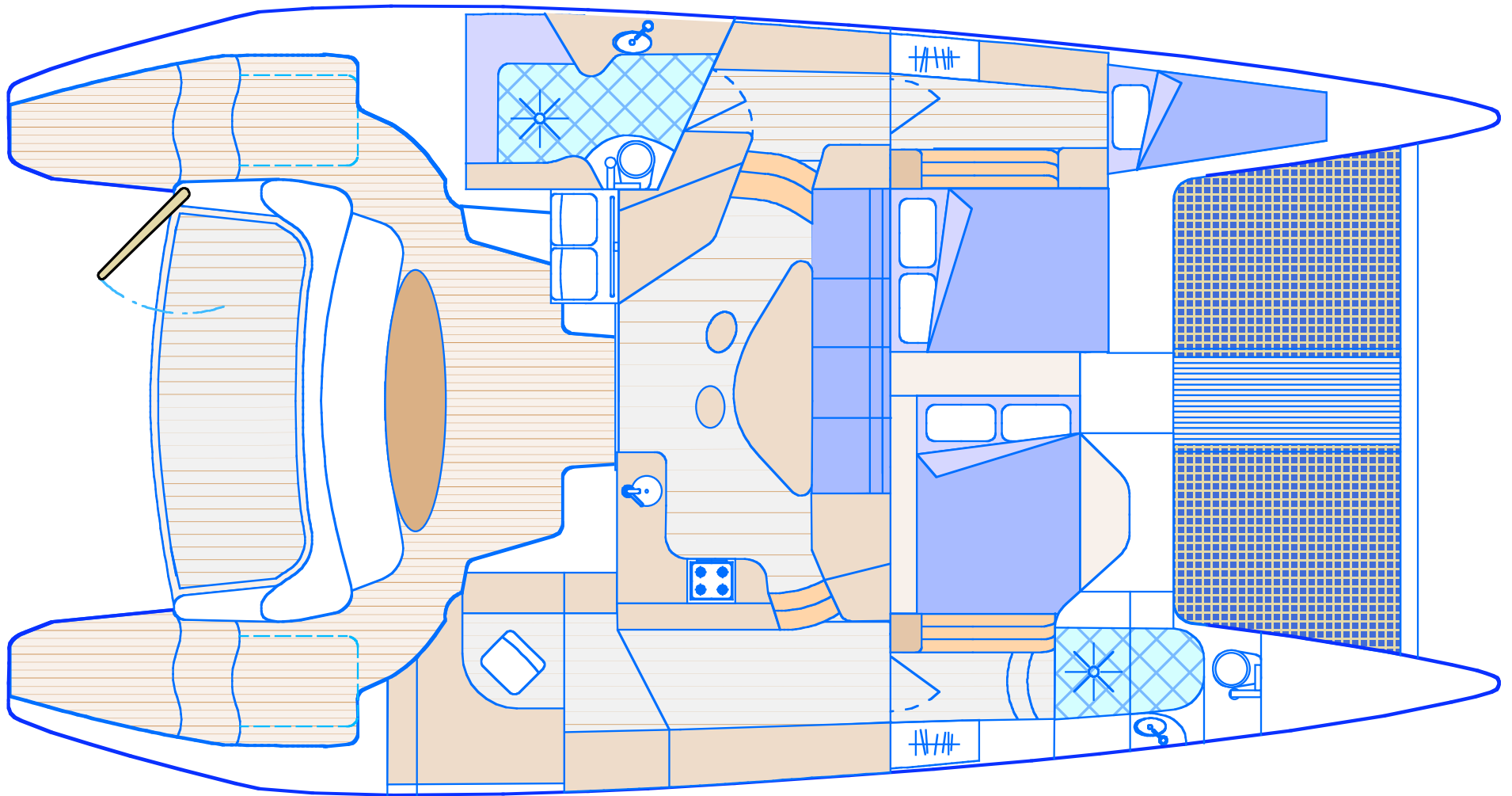
LIGHTWAVE 45 LAYOUT 3
