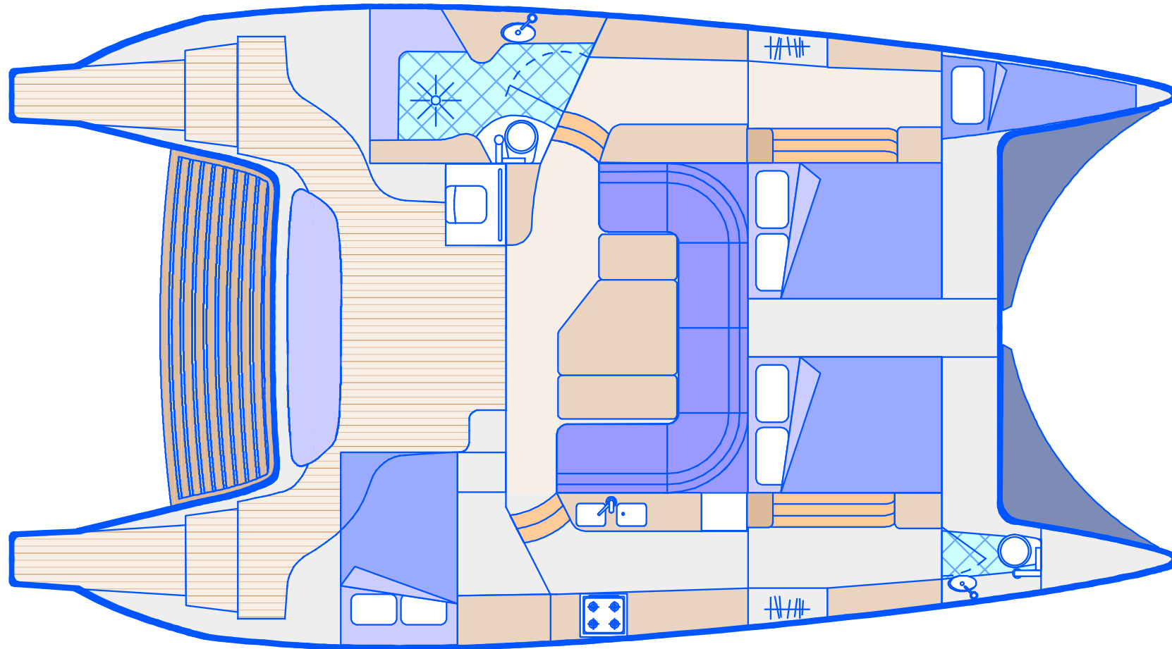
LIGHTWAVE 40 ACCOM OPTION -1 STANDARD LAYOUT WITH OPTIONAL FORWARD TOILET
