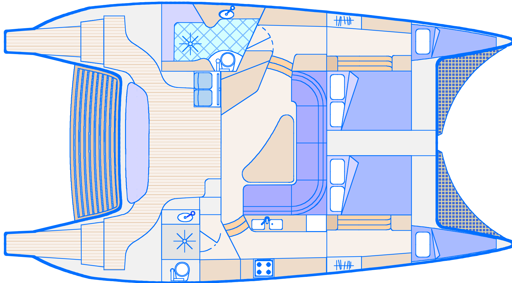
LIGHTWAVE 40 ACCOM OPTION -2 LARGE COMBINED NAV/ENTERTAINMENT AREA UPSTAIRS WITH DOUBLE HELM SEAT AND 2ND SHOWER/TOILET OPTION
