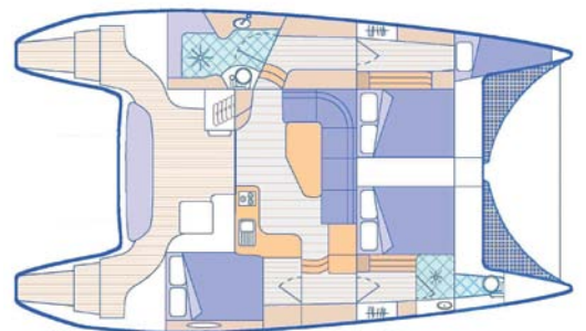
Charter Layout, Galley Up with Extended Aft Cabin
