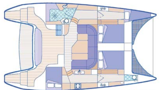
Family Layout with Duckboard
