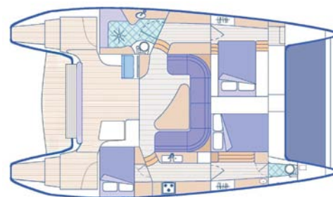
Custom Layout with Fwd Master Cabin, End Mounting Bed configuration; Raised Transom Seat; Duckboard
